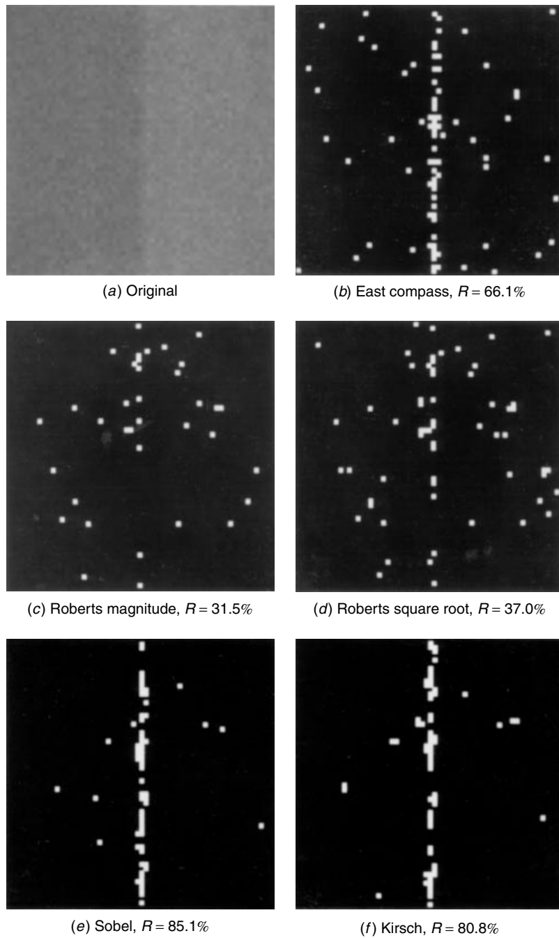
FIGURE 15.5-14. Edge location performance of several edge detectors for SNR = 10, h = 0.1 , w = 1 , a = 1/9 .
